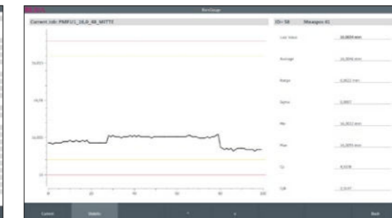
Statistical analysis
