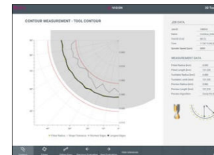
Visualisation of the measurement results of a ball cutter
